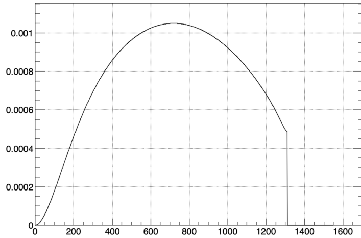
^{40}\text{K}
