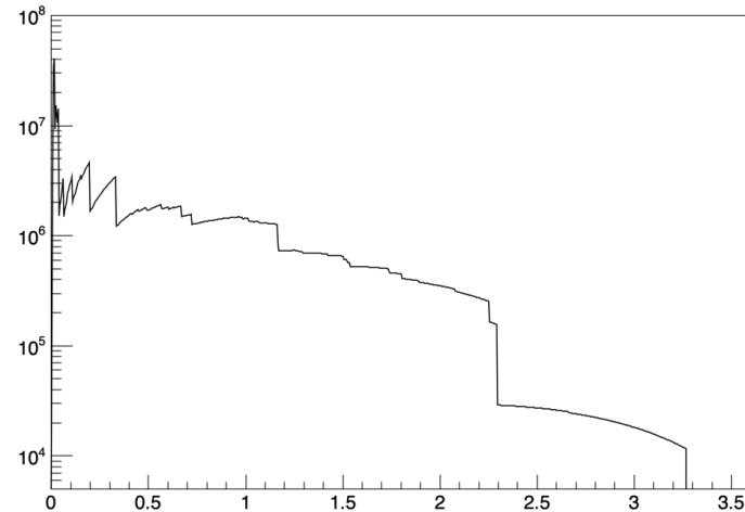
^{232}\text{Th}, ^{238}\text{U}
